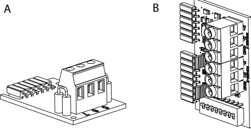
High Wall Connectivity Kit (only TA version)
